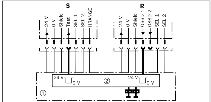
Fig. 5-8: Configuration of the cyclic system test, connection of the test input and the OSSD outputs
